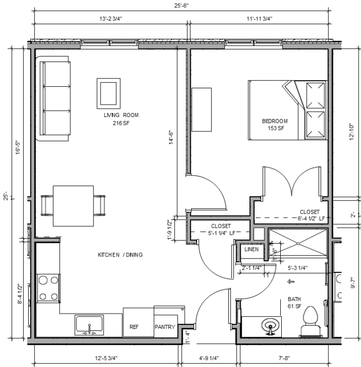
UNIT PLAN TYPE A
