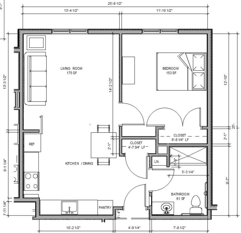
UNIT PLAN TYPE B
