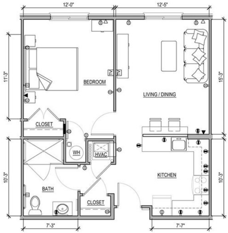
Typical Unit Plan
