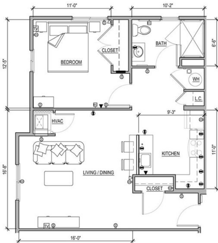
Typical End Unit Plan
